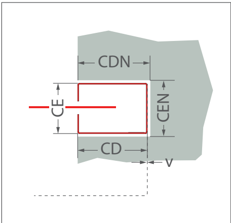
Recess mounting
