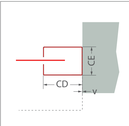
Soffit mounting
